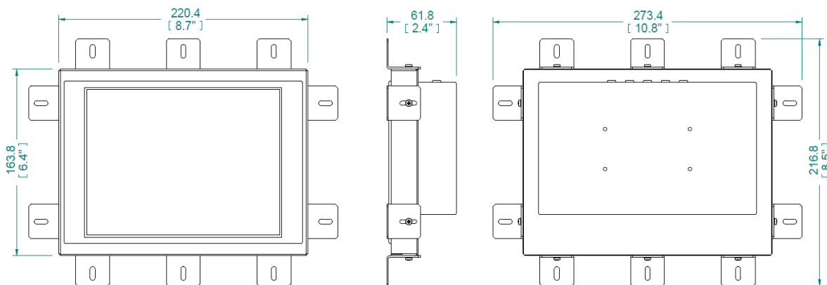
This image pertains to outlines only in mm (Inch). Download the dimensional drawing for detailed information.
