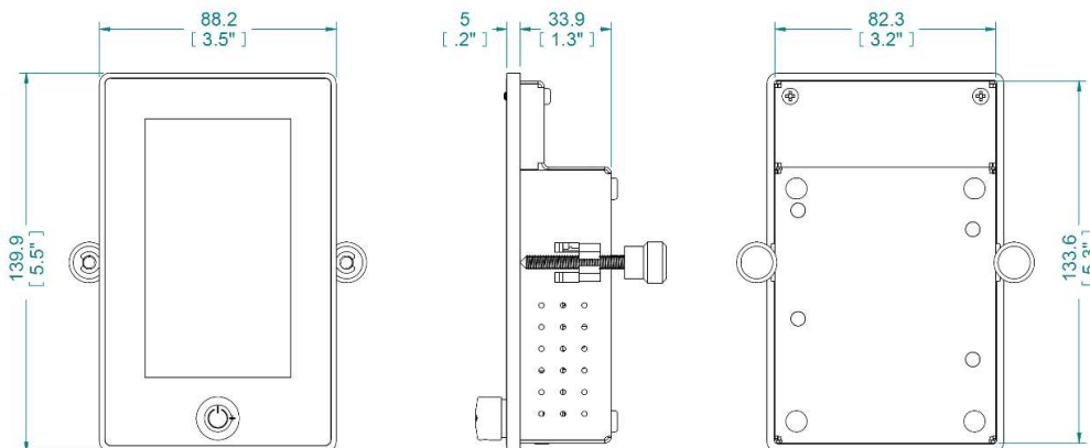
This image pertains to outlines only in mm (Inch). Download the dimensional drawing for detailed information.
