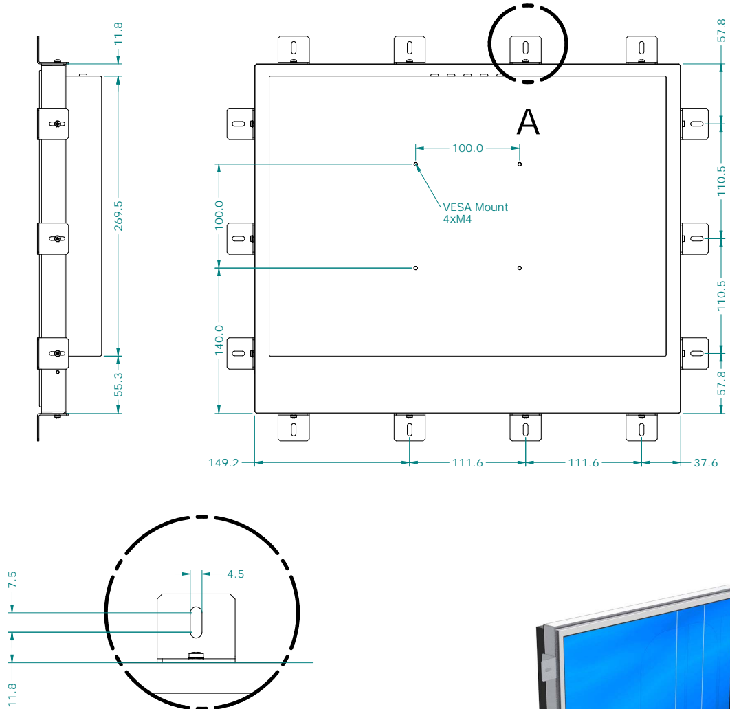
DETAIL A
